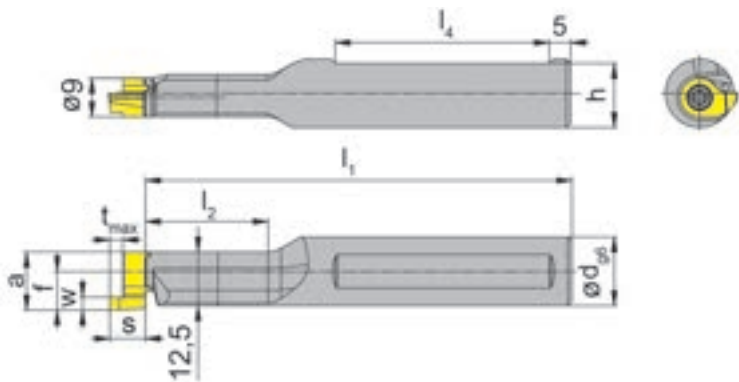
Abbildung = rechtsschneidend Picture = right hand cutting version
