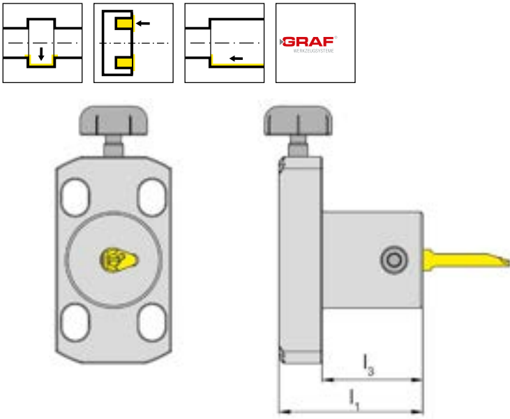
Abbildung = rechtsschneidend Picture = right hand cutting version
